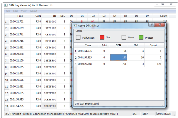
J1939 DTC-Viewer
