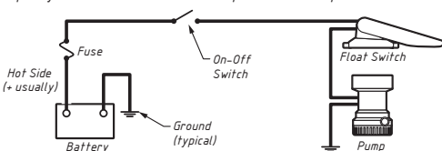
Best System - Provides Manual On/Automatic Control of the Pump and Red Light Indication of Operation
